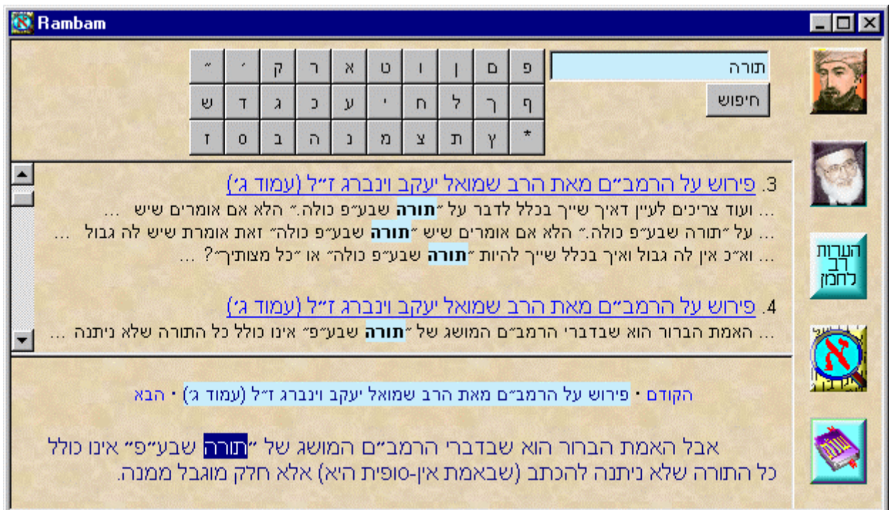
Search screen.
